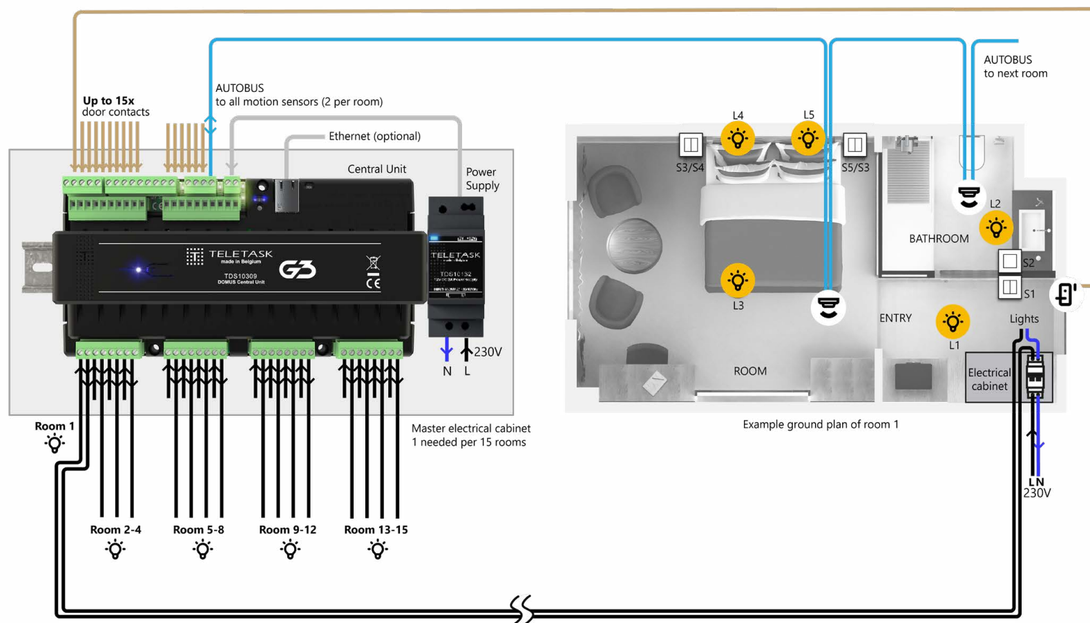
Example floor plan of 15 rooms
