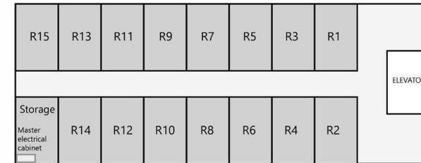
Example floor plan of 15 rooms
